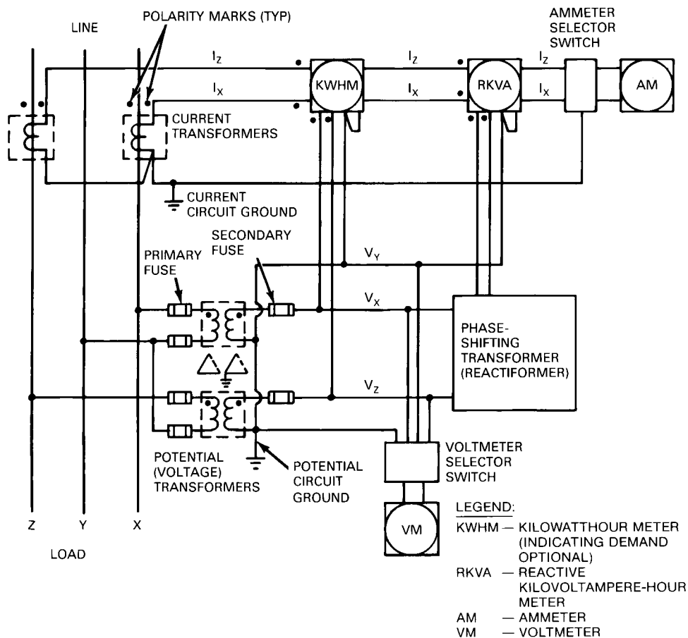
Figure 11-2—Sample metering scheme (3-phase, 3-wire, high current and voltage)
