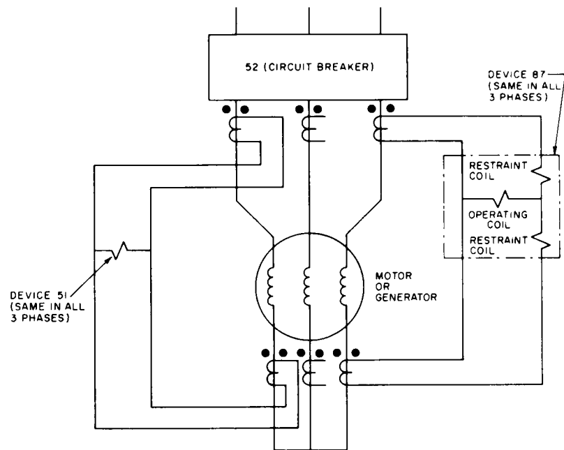
(a) Using percentage-type differential relays (Device 87) or time-delay overcurrent relays (Device 51)
