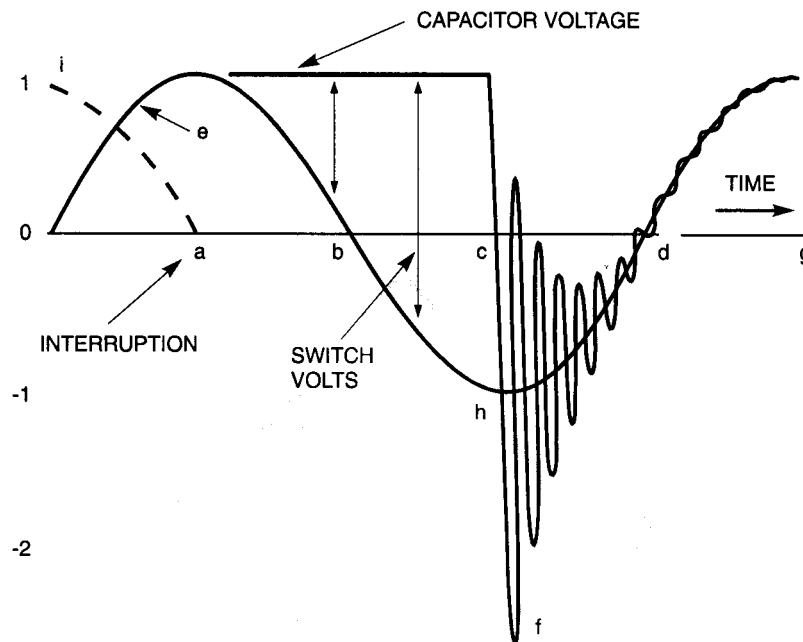
Figure 8-19—Capacitor de-energizing with a single maximum restrike following initial clearing
